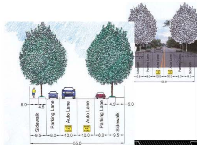
D Typical Cross Section Bladen Street and Duke Street
